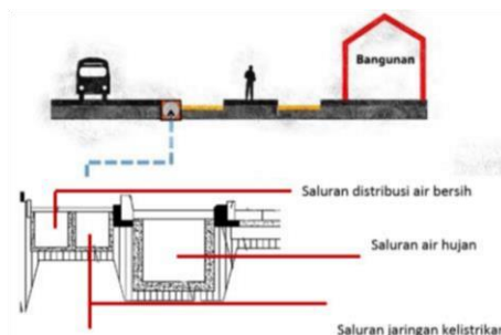
Gambar 10. Alur Distribusi Drainage Sistem
