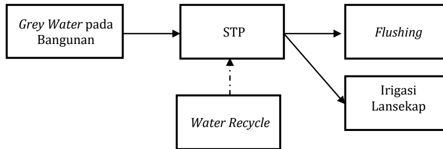
Gambar 6. Skema Daur Ulang Grey Water
